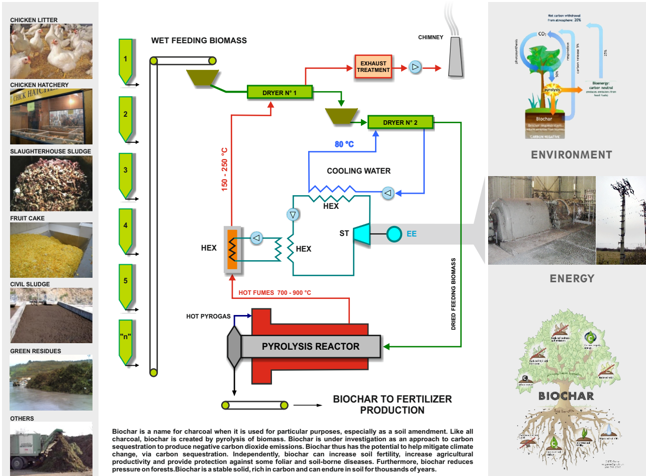
General scheme of pyrolysis by-products referred to different kind of biomass (Sohi, S - 2008)
