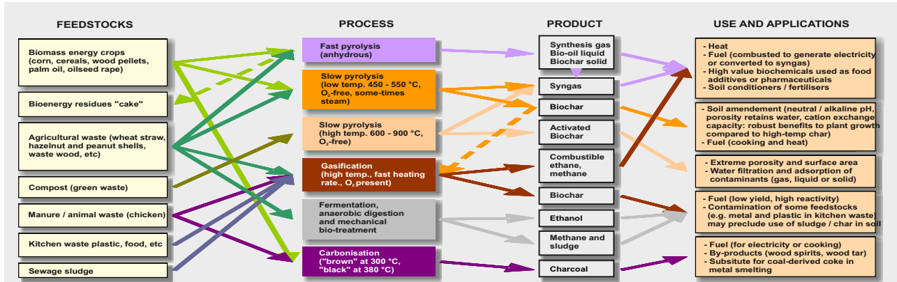
General scheme of pyrolysis by-products referred to different kind of biomass (Sohi, S - 2008)
